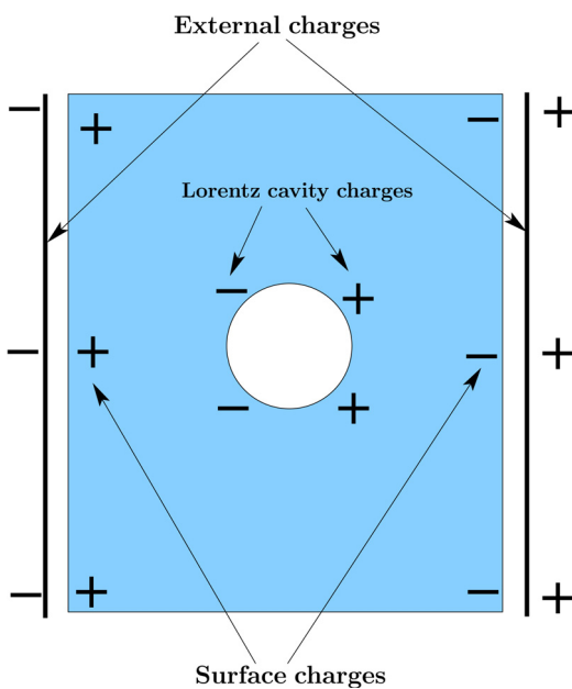
Figure 3.6. Illustrating the Lorentz cavity in the calculation of the dielectric constant of an insulator. The cavity has been created by scooping out a sphere of continuous dielectric having its center on an atom and a large radius.
