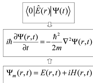
Fig. 2.2 Top Down: The time-dependent Schrödinger wave equation follows from the quantum optical “a photon is what a photodetector detects” definition. This is in accord with the usual wave function definition \Psi(\mathbf{r}, t) = \langle \mathbf{r} | \Psi(t) \rangle since |\mathbf{r}\rangle = \hat{\Psi}^+(\mathbf{r})|0\rangle . Bottom Up: The time-dependent Schrödinger wave follows nicely from the classical Maxwell equations by, for example, working with a combination of electric and magnetic fields
