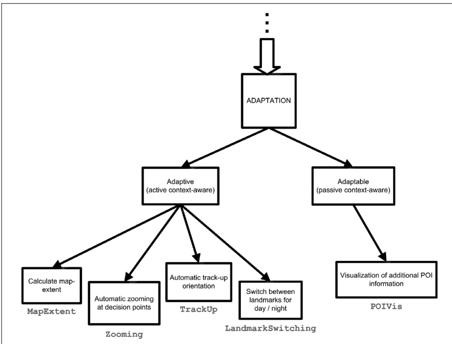
Fig. 2.6. Operations for mobile map adaptation in pedestrian navigation services. Automatic zooming at decision points.
