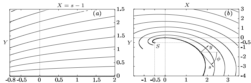
Fig. 2. Streamlines \psi = 0, 0.25, 0.5, \dots and wall contour (bold): (a) \Lambda = 0 , (b) \Lambda = 1
