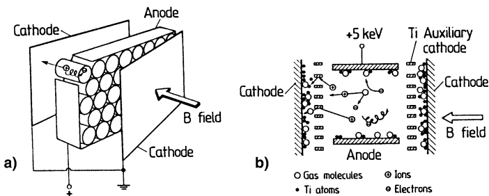
Fig. I.7 (a), (b) Schematic view of an ion-getter pump: (a) The basic multicell arrangement. Each cell consists essentially of a tube-like anode. The cells are sandwiched between two common cathode plates of Ti, possibly together with auxiliary cathodes of Ti. (b) Detailed representation of the processes occurring within a single cell. Residual gas molecules are hit by electrons spiralling around the magnetic field B and are ionized. The ions are accelerated to the cathode and/or auxiliary cathode; they are trapped on the active cathode surface or they sputter Ti atoms from the auxiliary cathode, which in turn help to trap further residual gas ions
