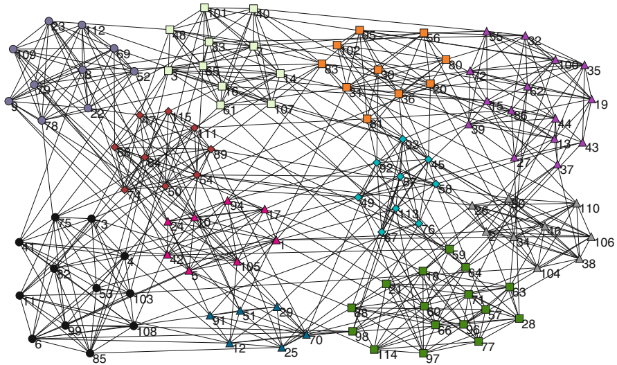
Fig. 1 Optimal clustering of network football obtained refining the NR heuristic result
