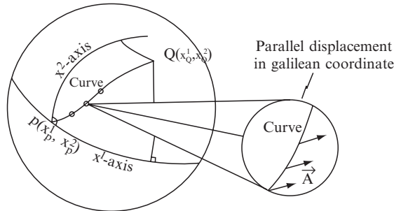
Fig. 2.1 Parallel displacement in curvilinear coordinates.
